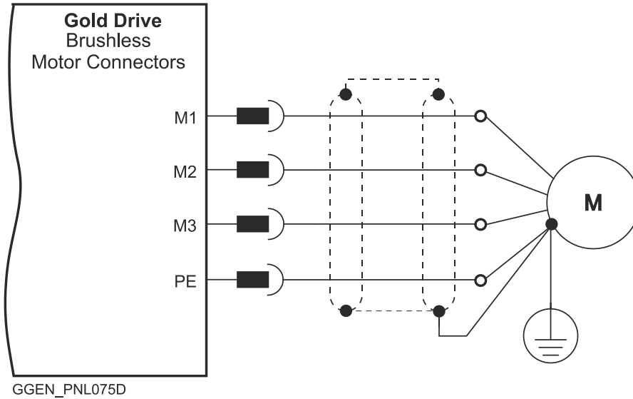
Figure 12: Brushless Motor Power Connection Diagram
