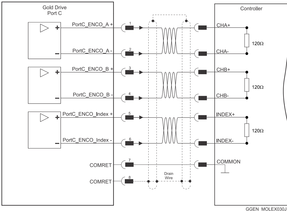
Figure 25: Encoder Differential Output – Recommended Connection Diagram
