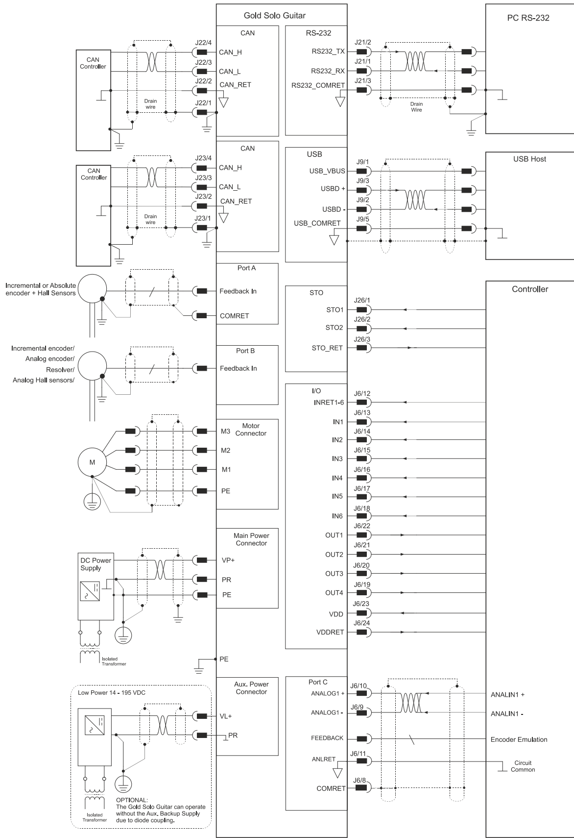
Figure 5: The Gold Solo Guitar Connection Diagram – CAN
