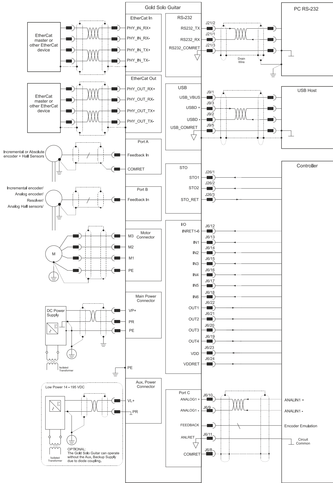
Figure 4: The Gold Solo Guitar Connection Diagram - EtherCAT
