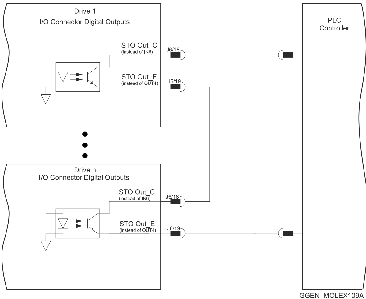
Figure 35: STO Output
