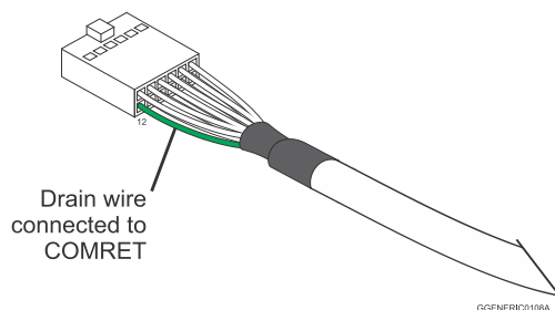
Figure 6: Feedback and Molex Control Cable Assemblies
