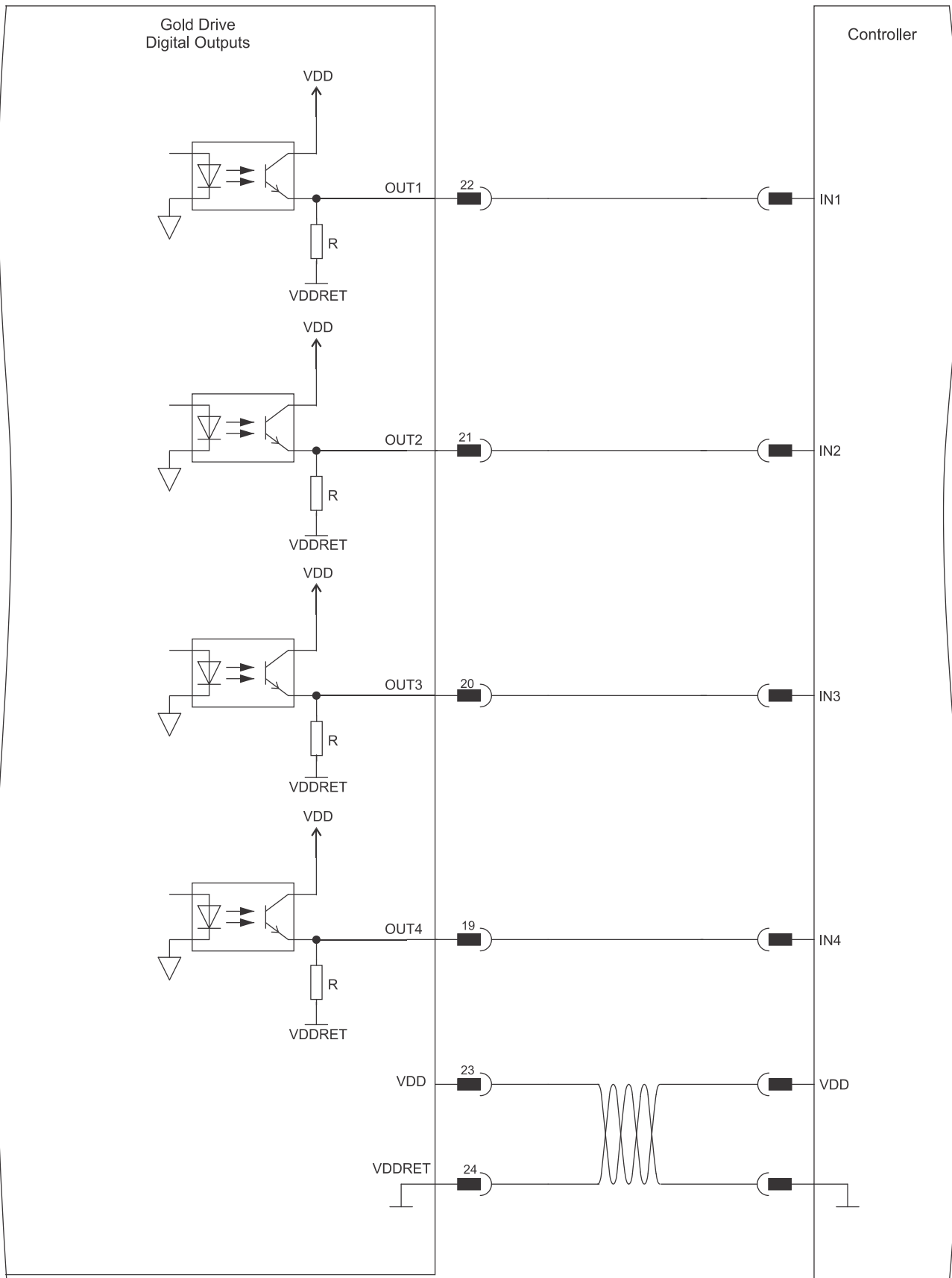
Figure 28: Digital Output Connection Diagram – TTL Option
