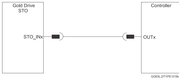
Figure 11: STO Cable Assemblies
