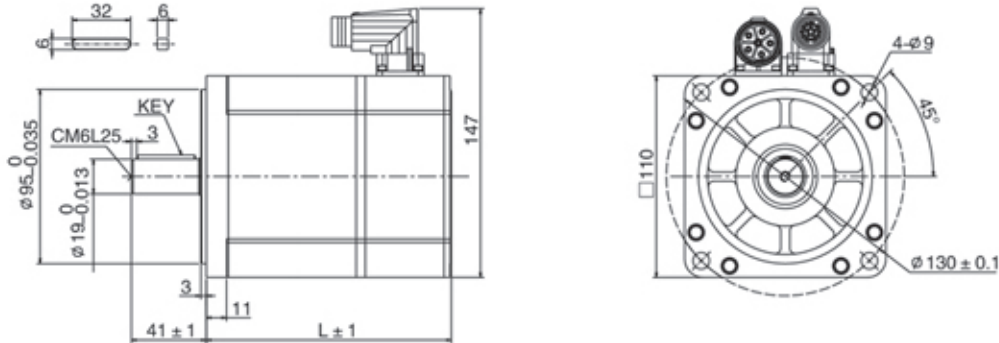
SMH110 D series Length
