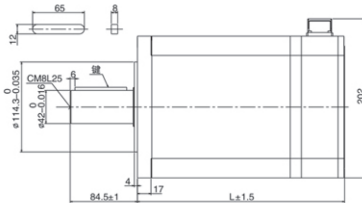
SMH180 M series Length (Unit: mm)
